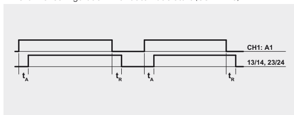
1-channel configuration with manual start (CS AR-40)
