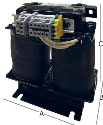
Model: XHP, 2-5kVA, vertical.
