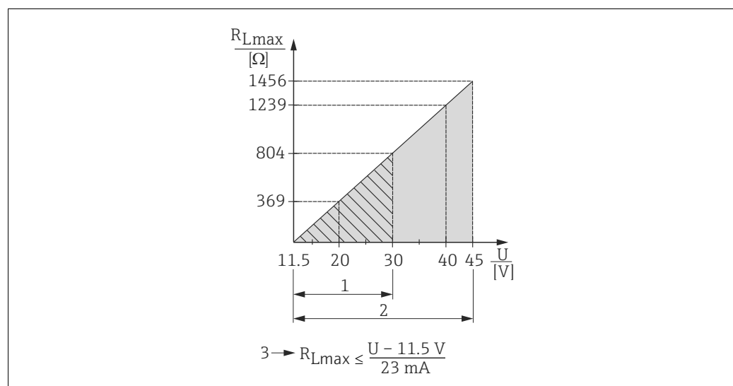
Load diagram
