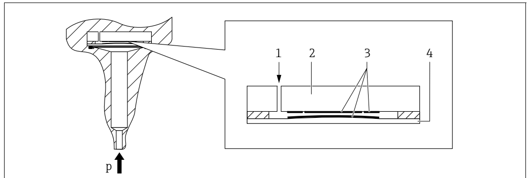
Ceramic sensor
