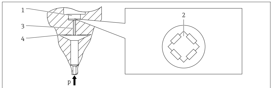
Metallic sensor
