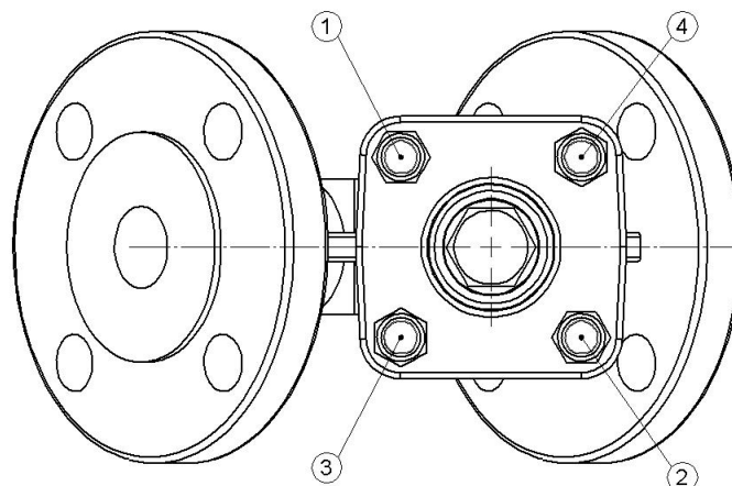
Tighten sequence of body – cover bolt nuts
