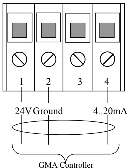
Terminal diagram
