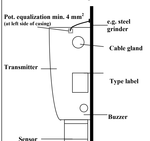
Potential equalization
