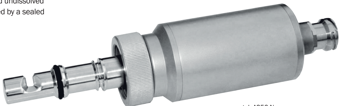
optek AS56-N Single Channel Absorption Probe
