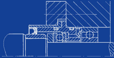
Shaft seal in a spindle boring head type HN 2390, friction-optimized.
