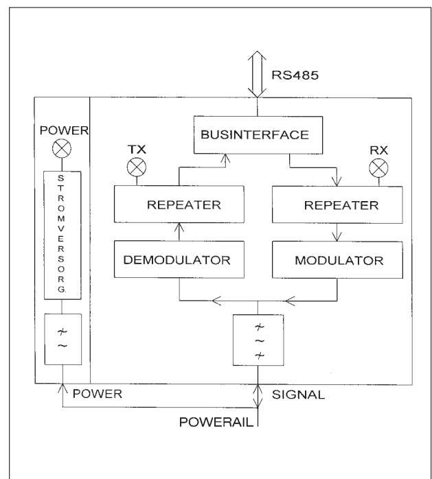
Block diagram
