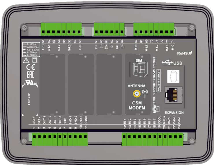
Backpanel view
