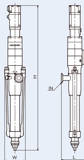
Type NDL dimensional outline drawing
