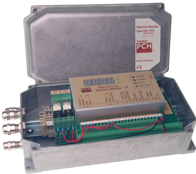
PCH 1072 Mk2 in enclosure with options
