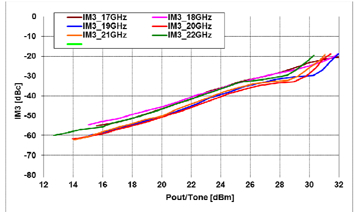
IM3 Level [dBc] vs. output power/tone [dBm] @Vds=6V, Idsq=2.5A
