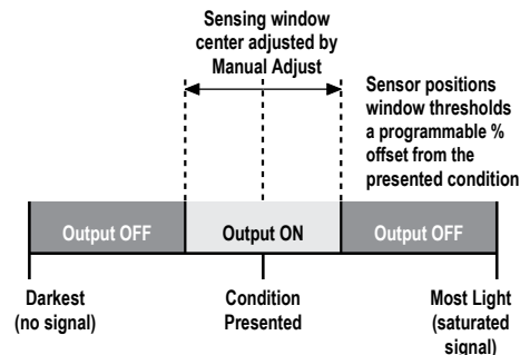
Figure 6. Window SET (Light Operate shown)
