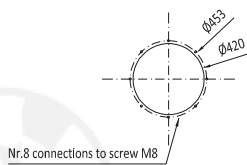
INLET FLANGE DETAIL
