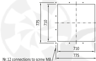
OUTLET FLANGE DETAIL
