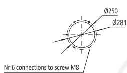
INLET FLANGE DETAIL
