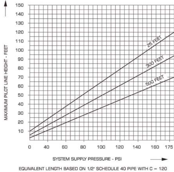
WET PILOT SPRINKLER HEIGHT LIMITATION OF 100 NB
