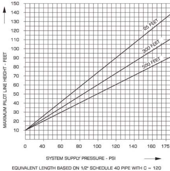
WET PILOT SPRINKLER HEIGHT LIMITATION OF 80 NB
