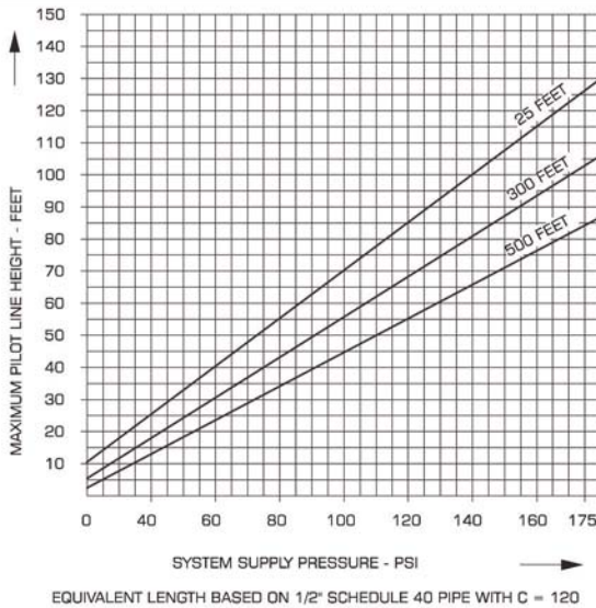
WET PILOT SPRINKLER HEIGHT LIMITATION OF 80 NB
