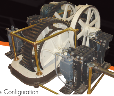
Dual Disc Brake Configuration
