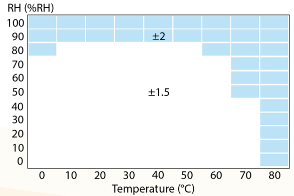
Typical Tolerance of RH over T
