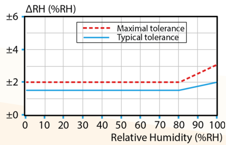
Tolerance of RH at 25°C
