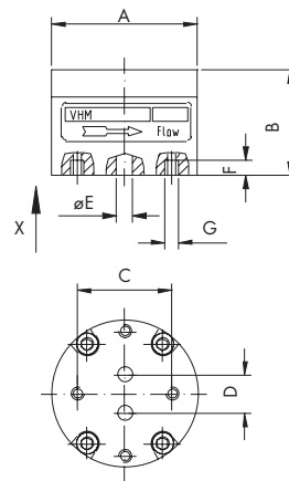
View X
