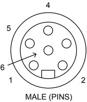
MALE (PINS)
