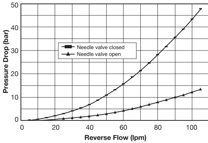
Typical Pressure Drop CK2FV2V Series (in reverse direction)
