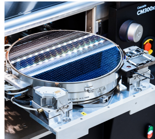
Pull-out chuck with OptoVue Pro in the auxiliary chuck position - CM300xi
