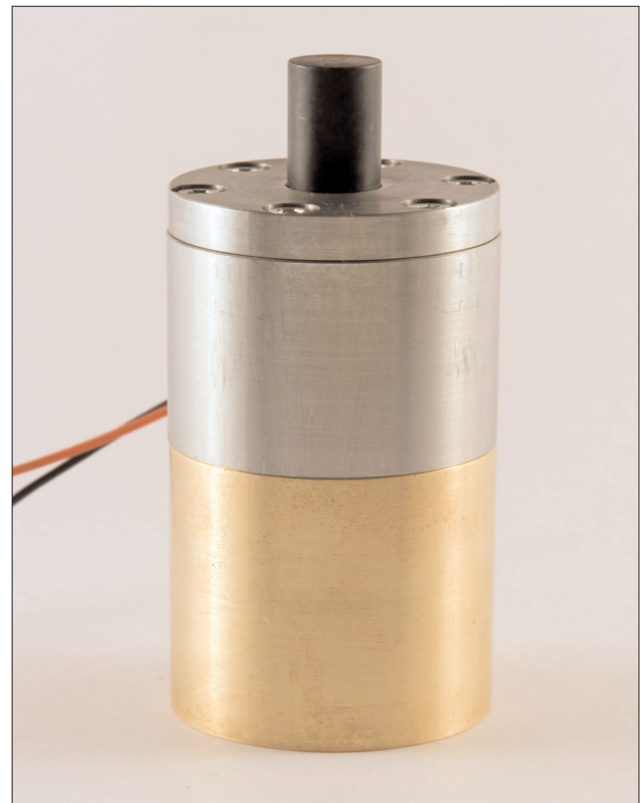
Figure 6b: Single output piezo-shock-generator: brass part: seismic countermass.
