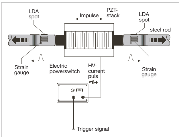
Figure 3: Symmetrical piezo-shock-generator with two-sided shock propagation. The shock parameters are detected by strain gages and LDAs.
