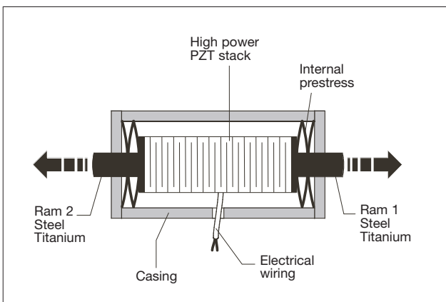
Figure 4a: Schematic of a symmetrical piezo-shock-generator.
