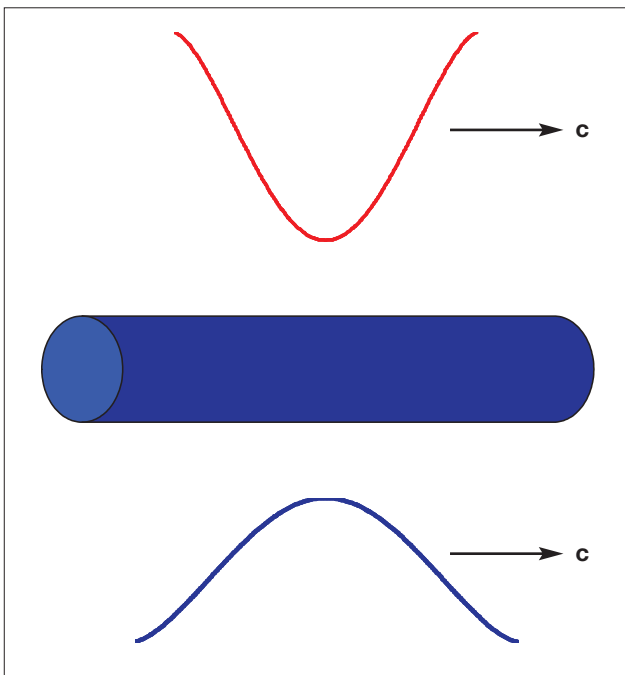
Figure 12: Stress impulse (top) and related particle velocity (bottom).
